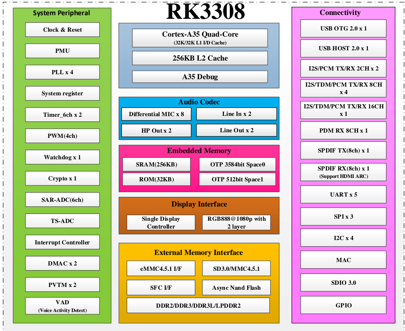
Fig.1-1 Block Diagram
