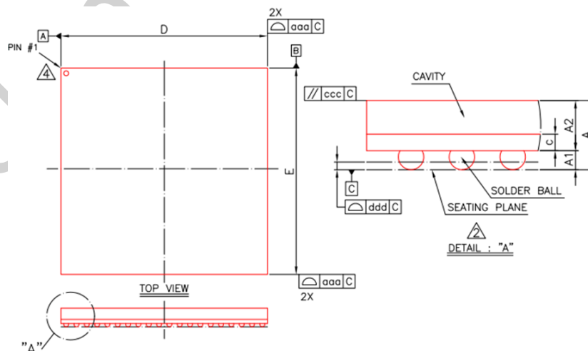
Fig.2-2 Package Top View and Side View
